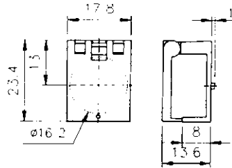
TN16-Round/Square Protection Cover TN16-GS @ n/a
