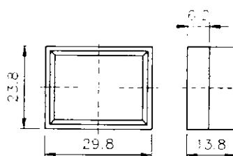
Rectangular Head Dust-Tight Cover TN16-WL @ n/a
